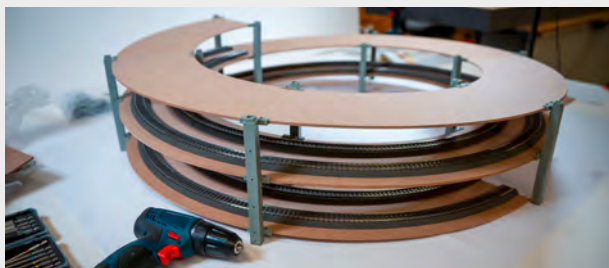
With additional assembly circles, the helix can be easily extended upwards.
