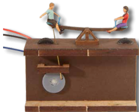
H0 13400 micro-motion Seesaw 5.6 cm x 4.5 cm x 5.5 cm installation depth 3.5 cm
