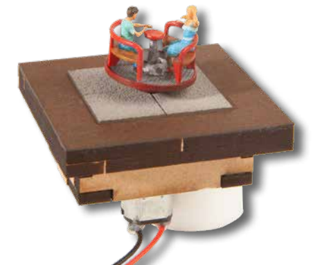
H0 13403 micro-motion Roundabout 5 cm x 5 cm x 5.4 cm installation depth 3.5 cm
